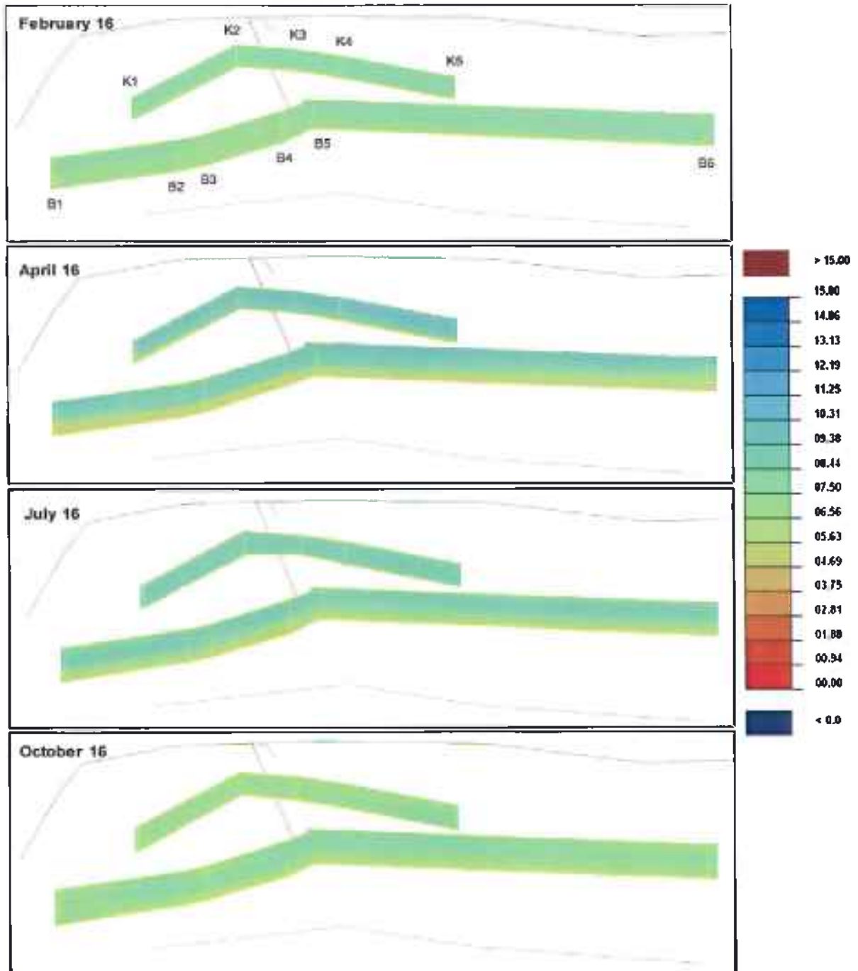
Figure 3-9. Dissolved oxygen contours for the K Station (depth = 18 m) and B Station (depth = 28 m) transects. The Goleta Sanitary District outfall is depicted as a red line.
