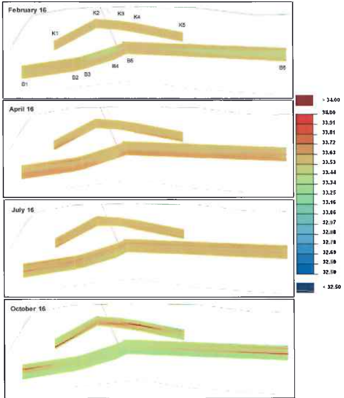
Figure 3-7. Salinity (ppt) contours for the K Station (depth = 18 m) and B Station (depth = 28 m) transects. The Goleta Sanitary District outfall is depicted as a red line.
