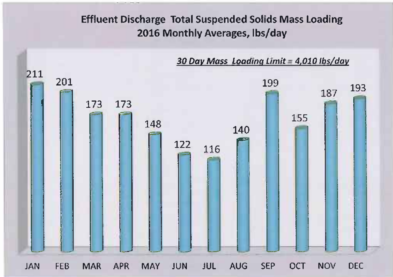
Figure 2-4. Effluent Discharge Total Suspended Solids Mass Loading, 2016 Monthly Averages, lbs/day
