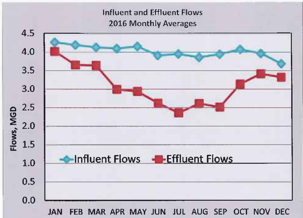
Figure 2-2. Influent and Effluent Flows 2016 Monthly Averages
