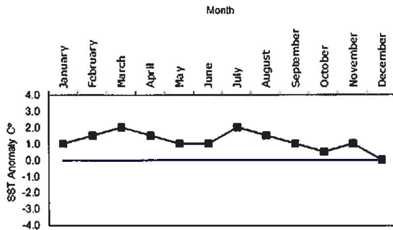
Figure 3-2. Sea surface anomaly temperatures for 2016 compared with long term trends.
