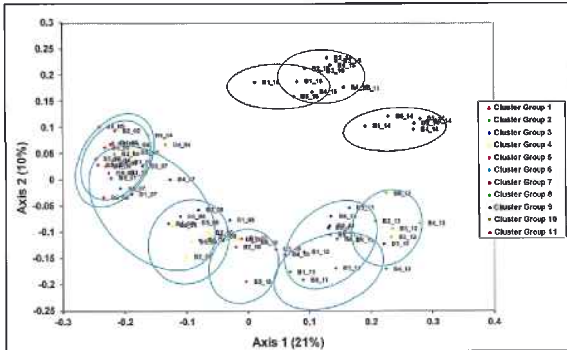
Figure 6-3. Plot of ordination scores for infauna communities at stations measured from 2004 to 2016.
