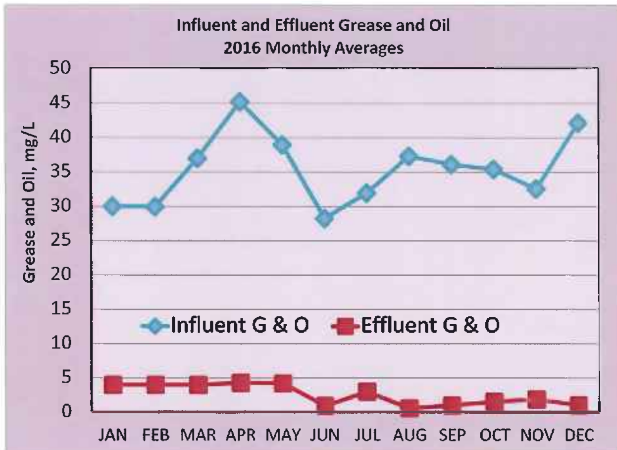
Figure 2-7. Influent and Effluent Grease and Oil 2016 Monthly Averages
