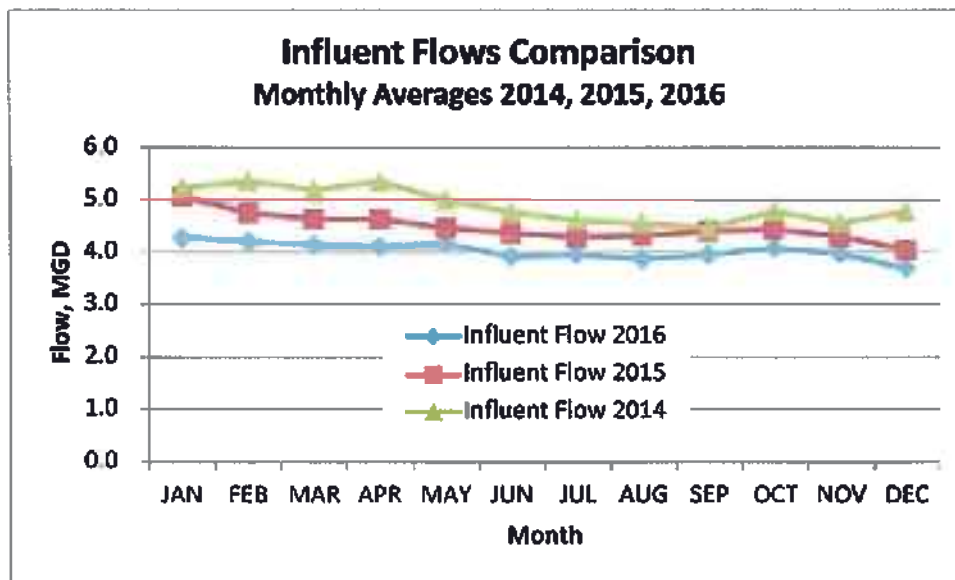
Figure 2-1. Influent Flows Monthly Average Comparison for 2014, 2015 and 2016
