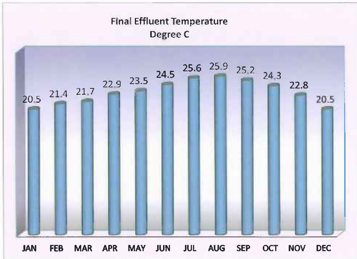
Figure 2-8. Effluent Discharge Temperature 2016 Monthly Averages
