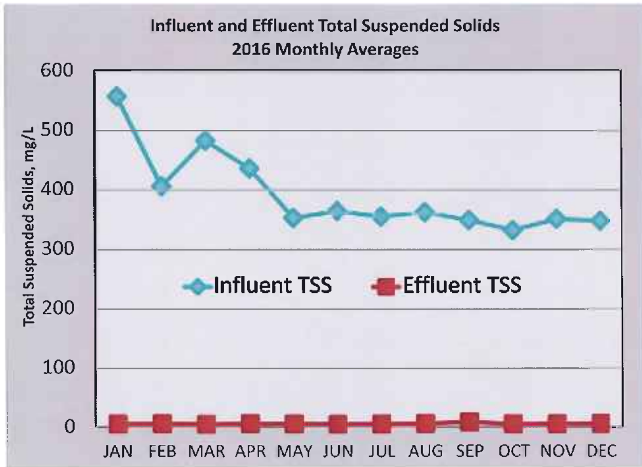
Figure 2-3. Influent and Effluent Total Suspended Solids 2016 Monthly Averages
