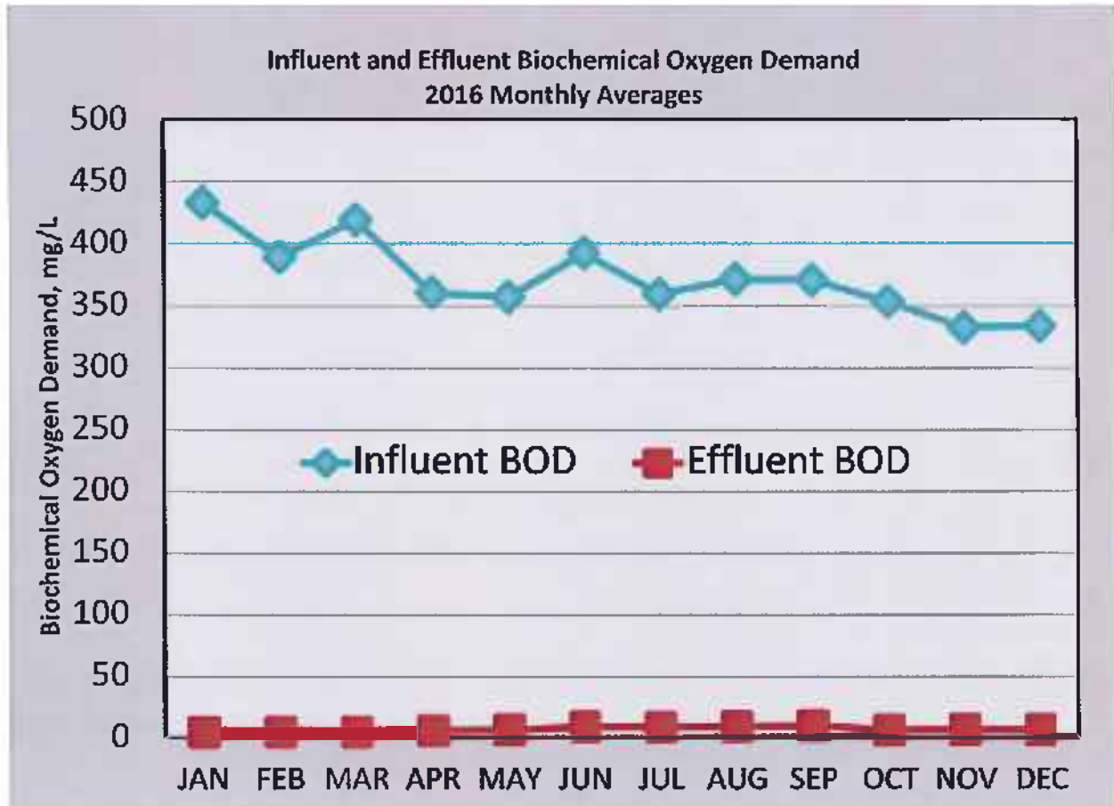
Figure 2-5. Influent and Effluent Biochemical Oxygen Demand 2016 Monthly Averages
