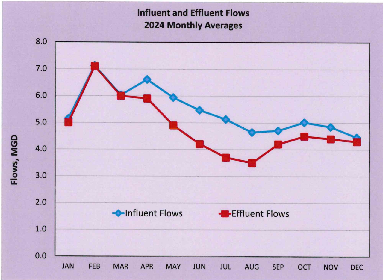
Figure 2-2. Influent and Effluent Flows 2024 Monthly Averages
