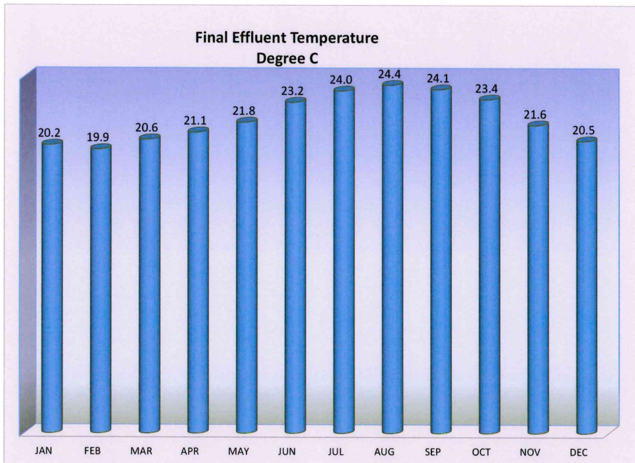
Figure 2-8. Effluent Discharge Temperature 2024 Monthly Averages
