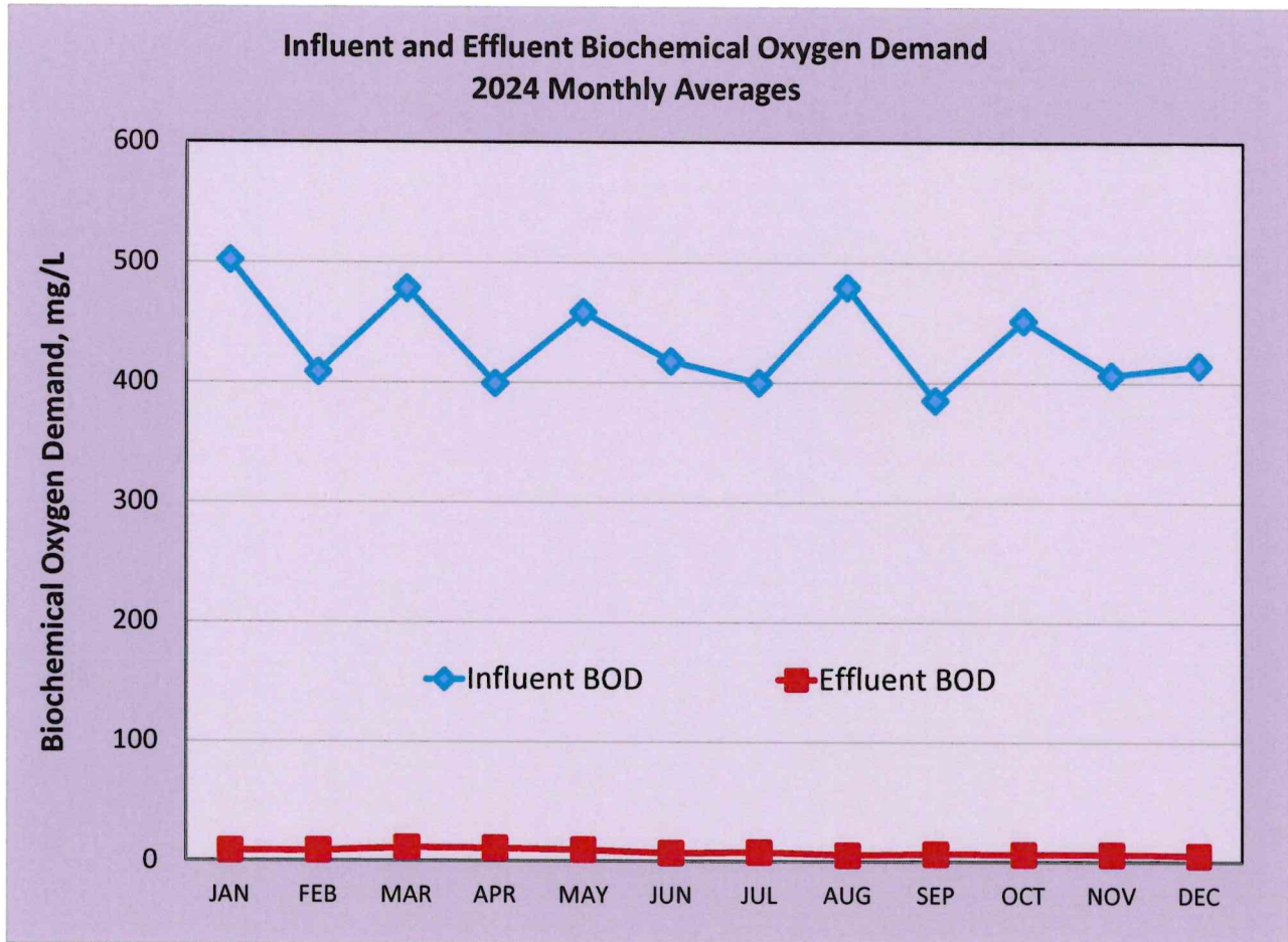
Figure 2-5. Influent and Effluent Biochemical Oxygen Demand 2024 Monthly Averages
