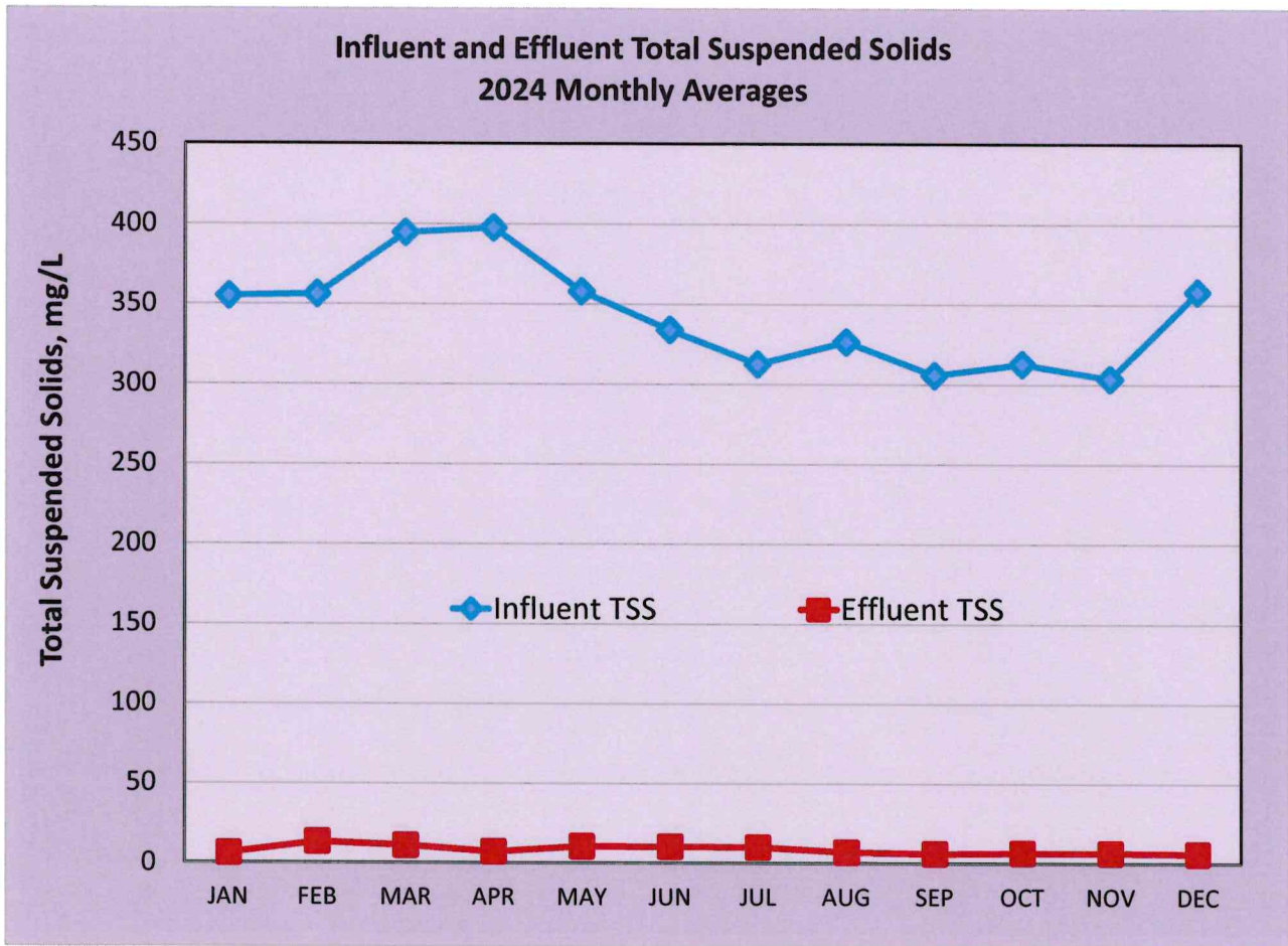
Figure 2-3. Influent and Effluent Total Suspended Solids 2024 Monthly Averages
