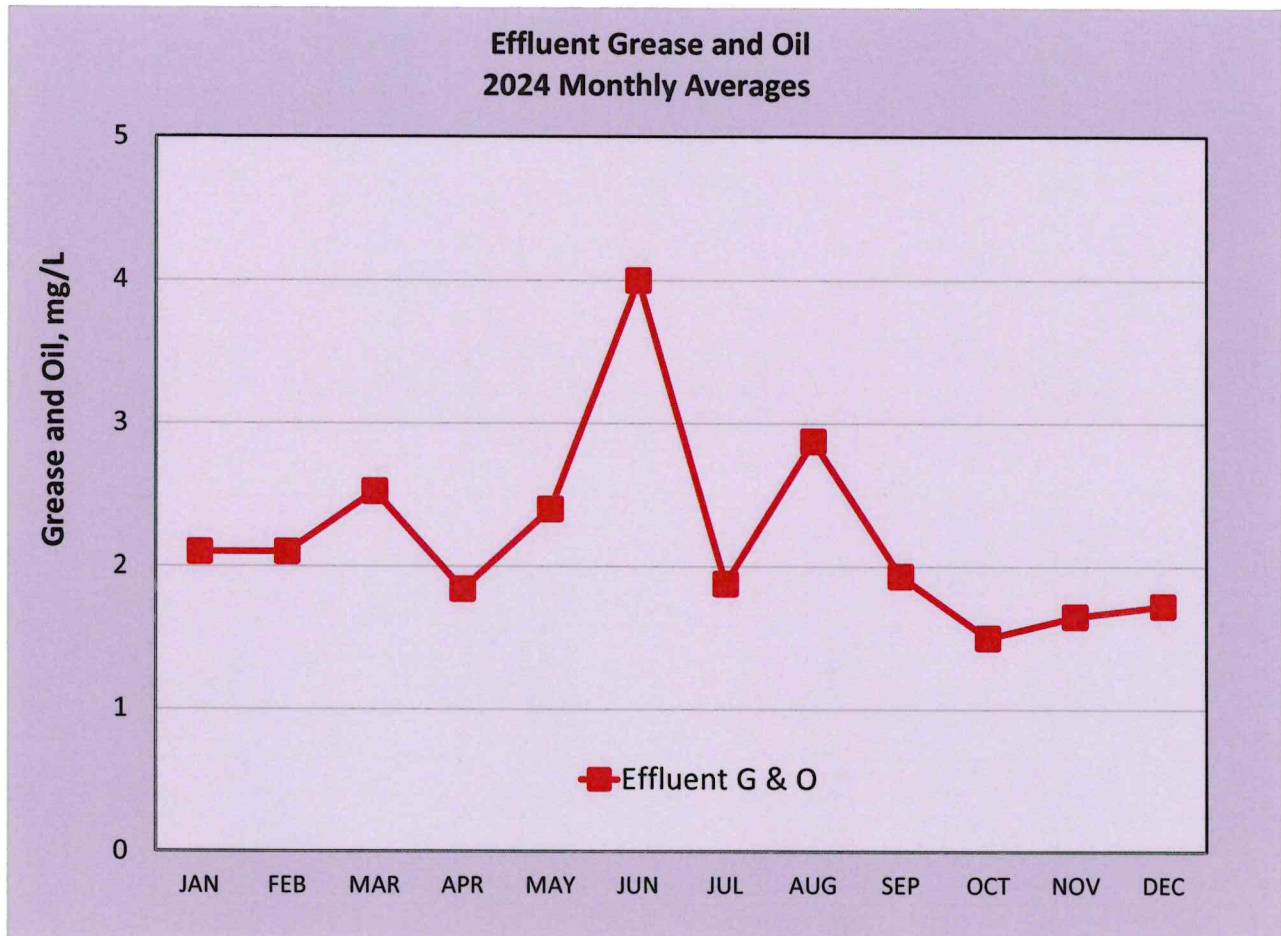
Figure 2-7. Effluent Grease and Oil 2024 Monthly Averages
