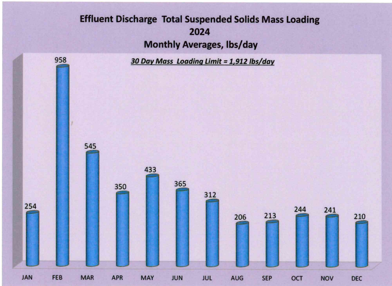
Figure 2-4. Effluent Discharge Total Suspended Solids Mass Loading, 2024 Monthly Averages, lbs/day
