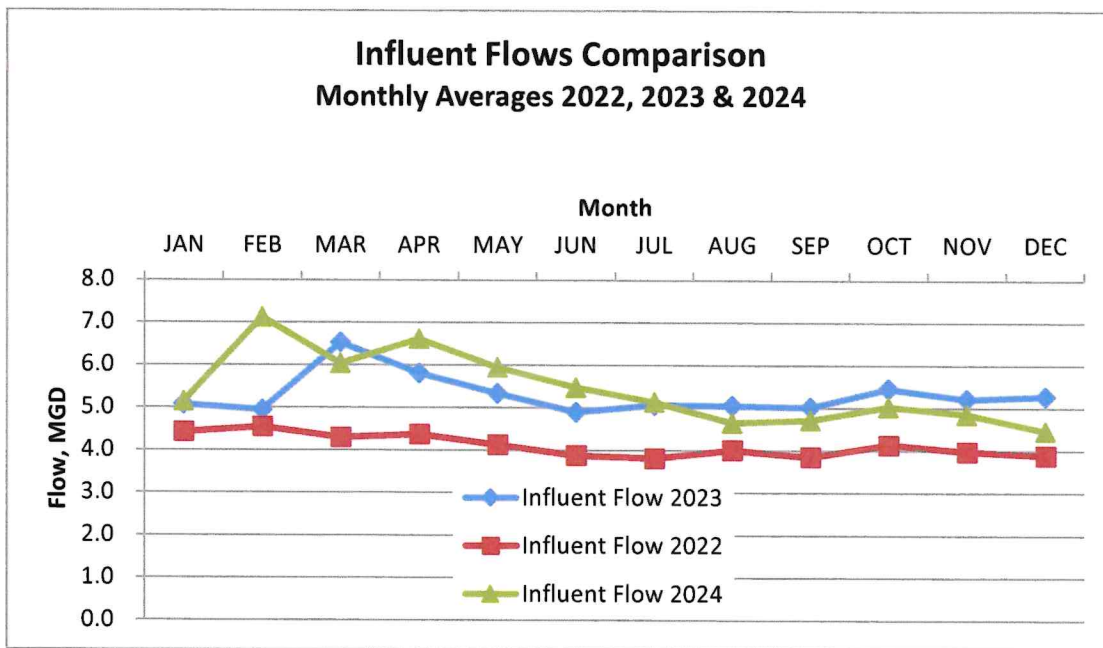
Figure 2-1. Influent Flows Monthly Average Comparison for 2022, 2023 and 2024
