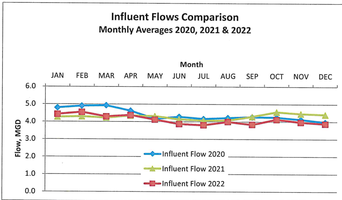
Figure 2-1. Influent Flows Monthly Average Comparison for 2020, 2021 and 2022
