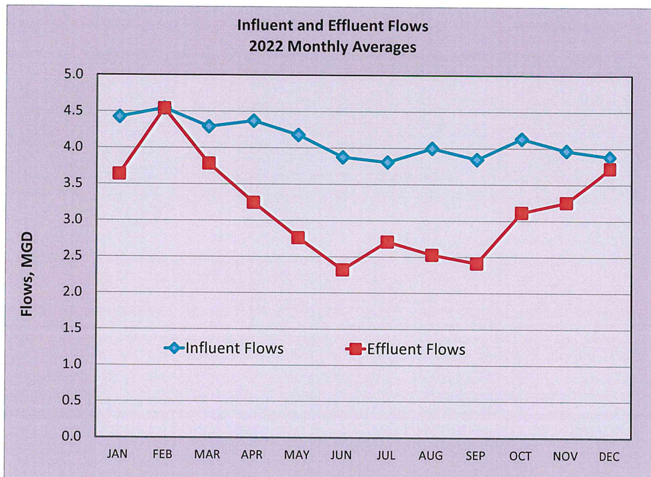
Figure 2-2. Influent and Effluent Flows 2022 Monthly Averages
