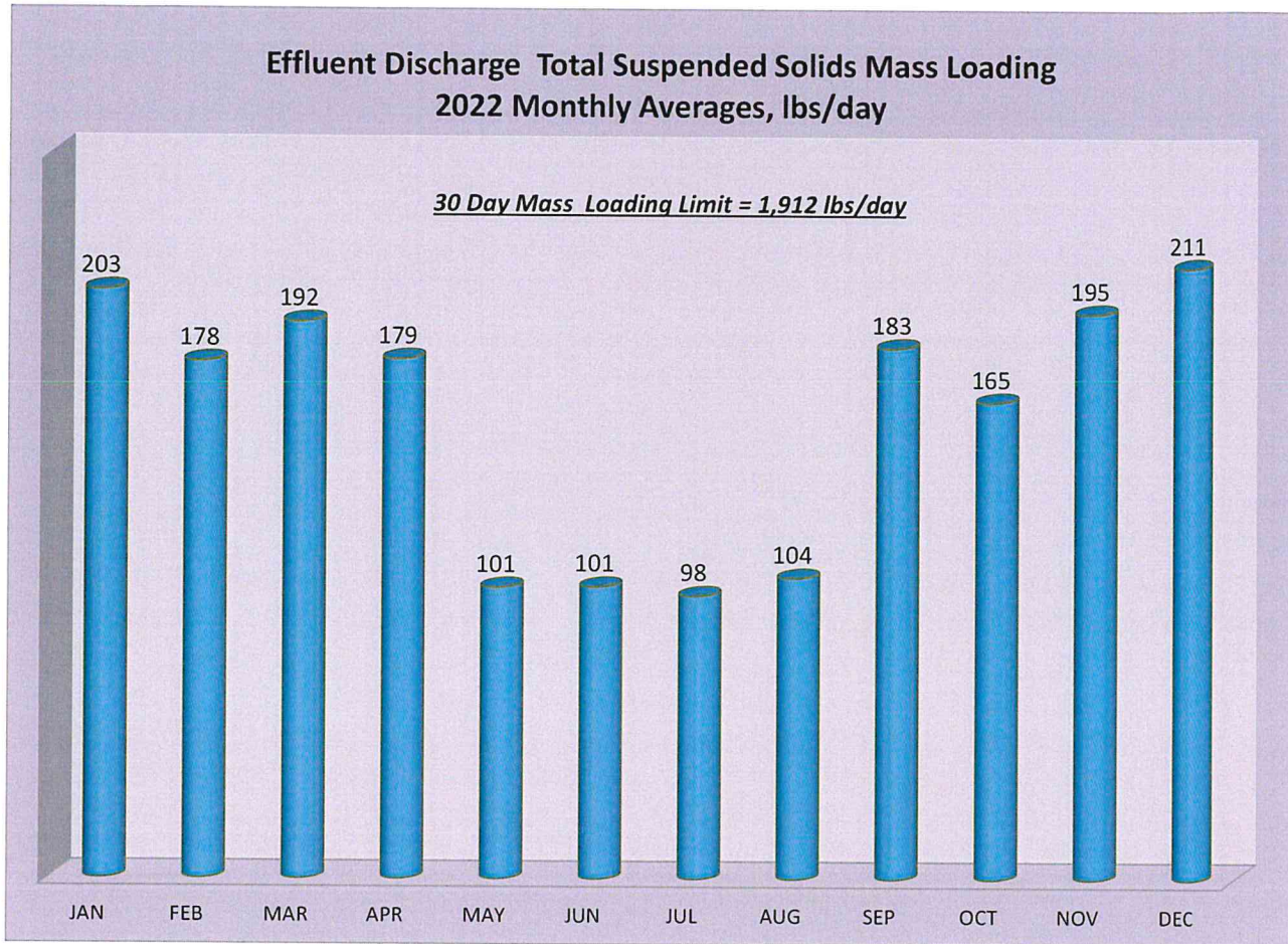
Figure 2-4. Effluent Discharge Total Suspended Solids Mass Loading, 2022 Monthly Averages, lbs/day
