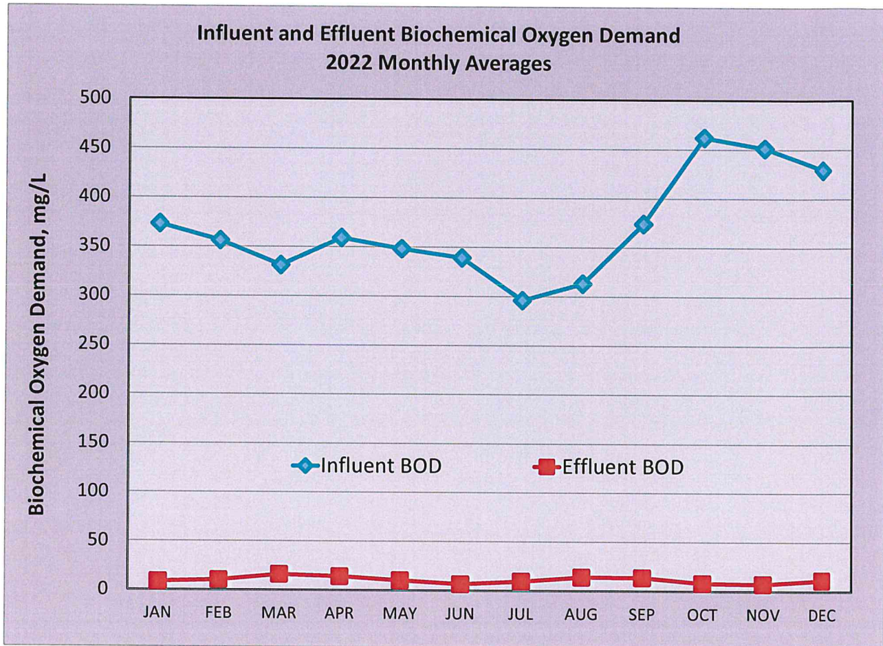
Figure 2-5. Influent and Effluent Biochemical Oxygen Demand 2022 Monthly Averages
