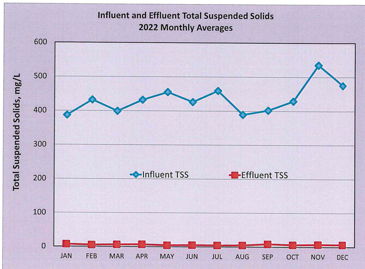
Figure 2-3. Influent and Effluent Total Suspended Solids 2022 Monthly Averages
