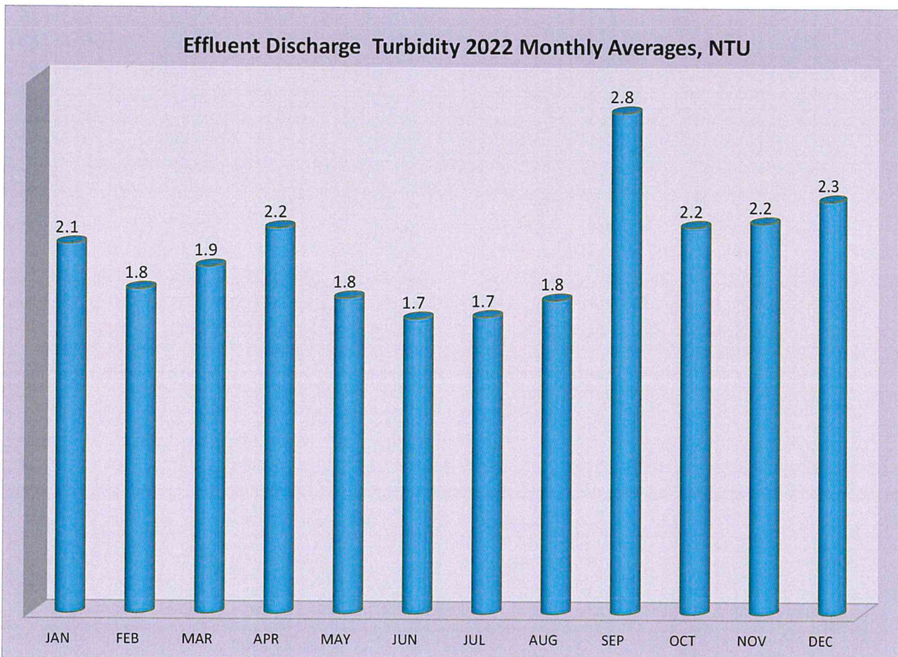
Figure 2-6. Effluent Discharge Turbidity 2022 Monthly Averages, NTU
