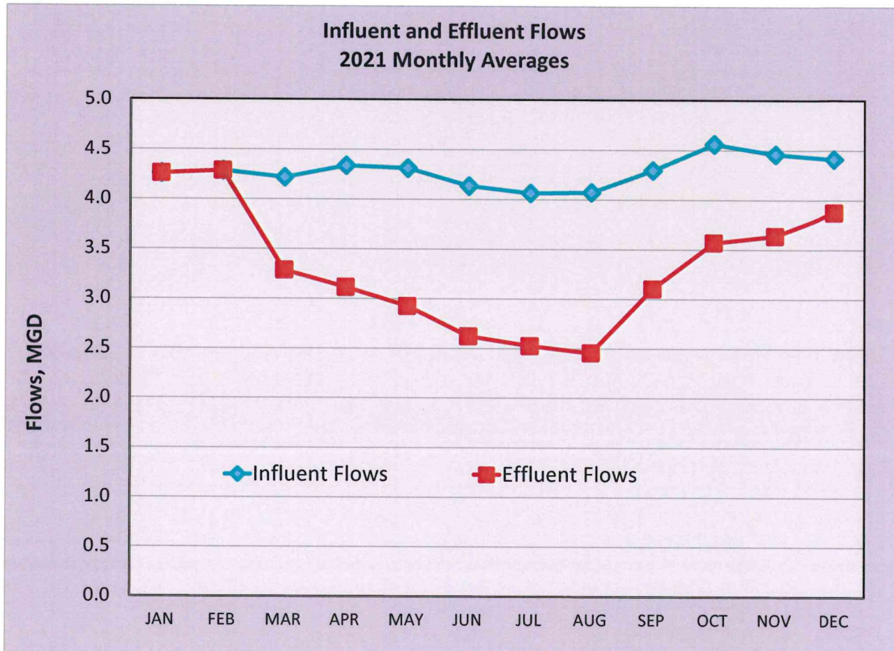
Figure 2-2. Influent and Effluent Flows 2021 Monthly Averages
