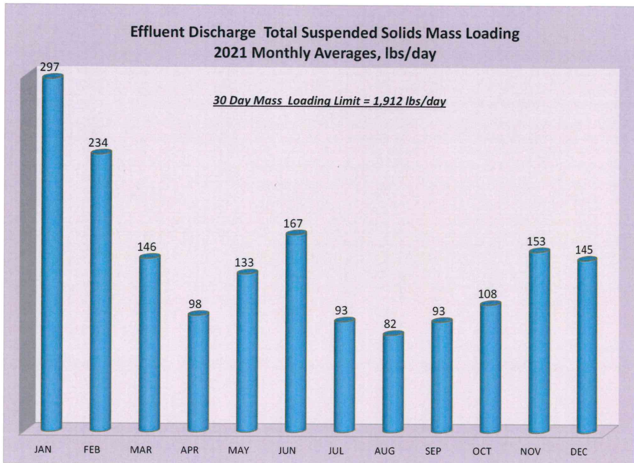
Figure 2-4. Effluent Discharge Total Suspended Solids Mass Loading, 2021 Monthly Averages, lbs/day
