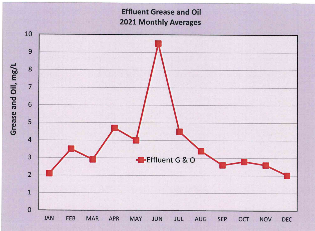
Figure 2-7. Effluent Grease and Oil 2021 Monthly Averages
