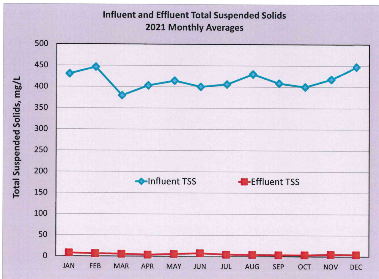
Figure 2-3. Influent and Effluent Total Suspended Solids 2021 Monthly Averages
