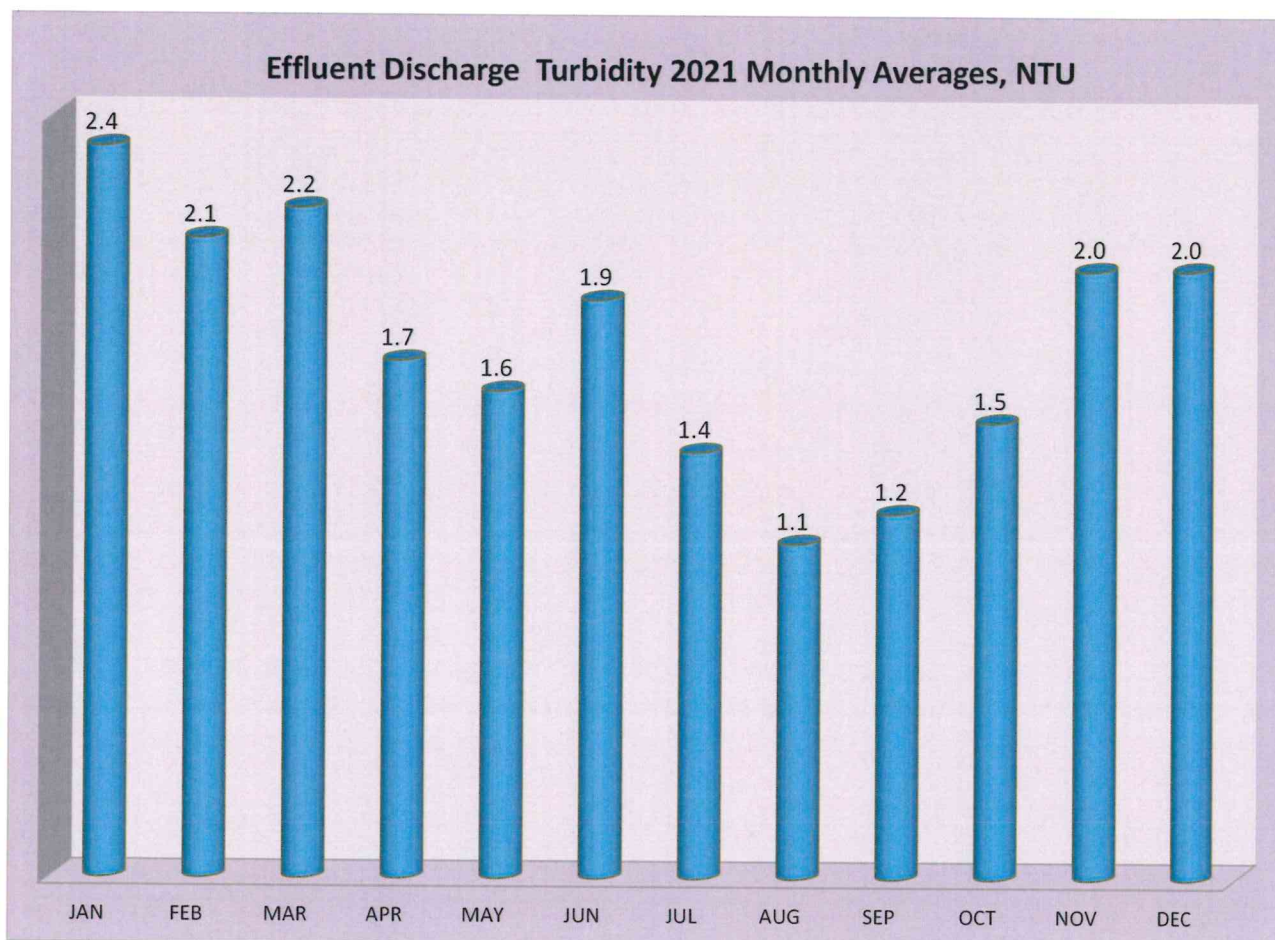
Figure 2-6. Effluent Discharge Turbidity 2021 Monthly Averages, NTU
