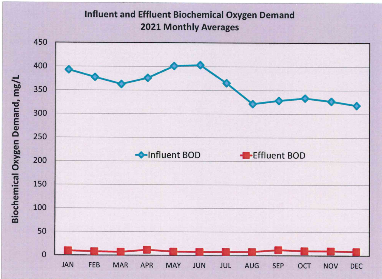
Figure 2-5. Influent and Effluent Biochemical Oxygen Demand 2021 Monthly Averages
